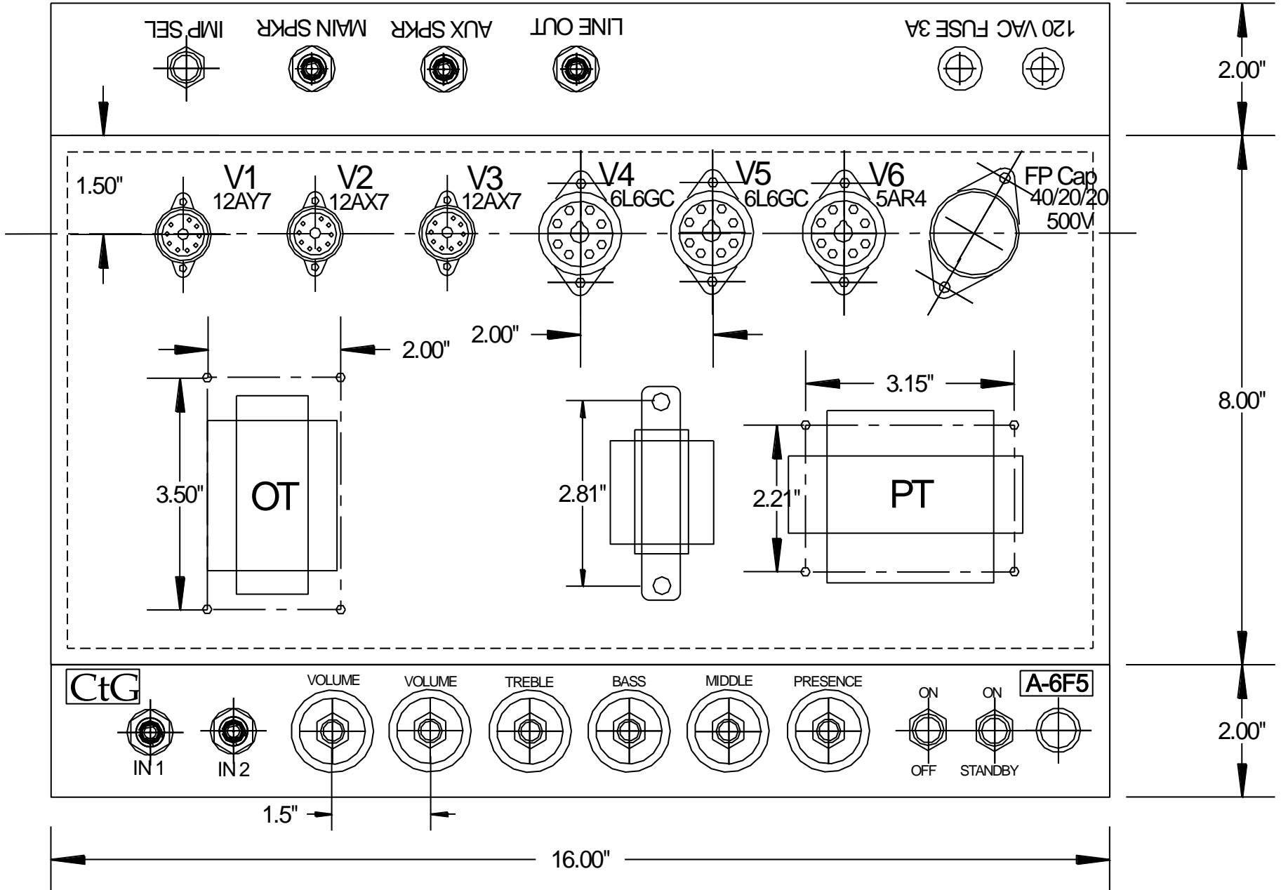
A-6F5 chassis rough layout CtG electronics k.b.c. 3/18/10
