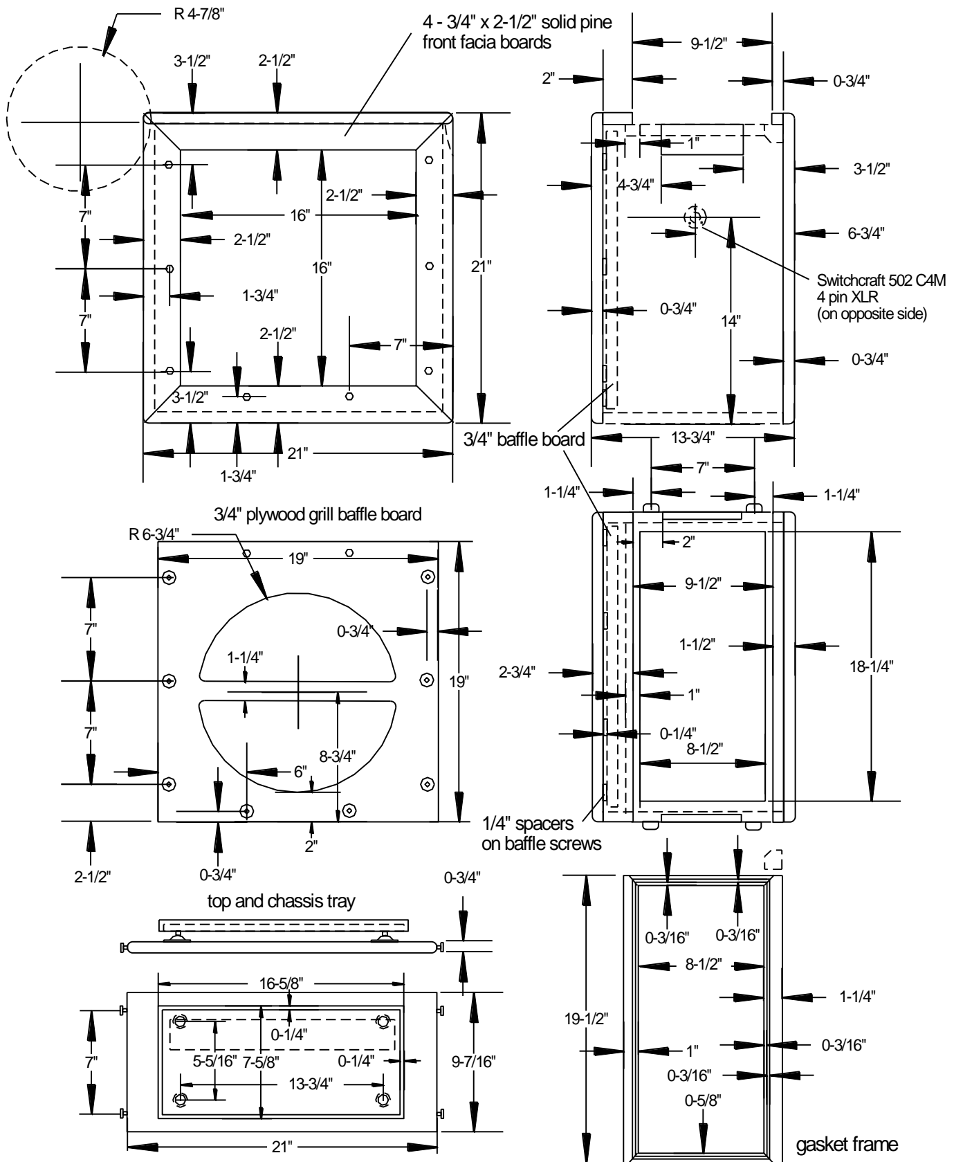
B-15NF single baffle cabinet
