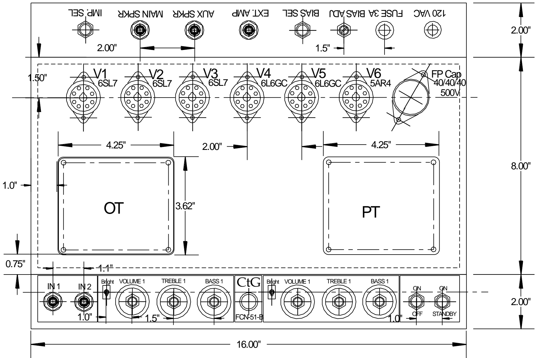
FCN-51-B amplifier chassis rough layout CtG electronics k.b.c. 2/14/10
