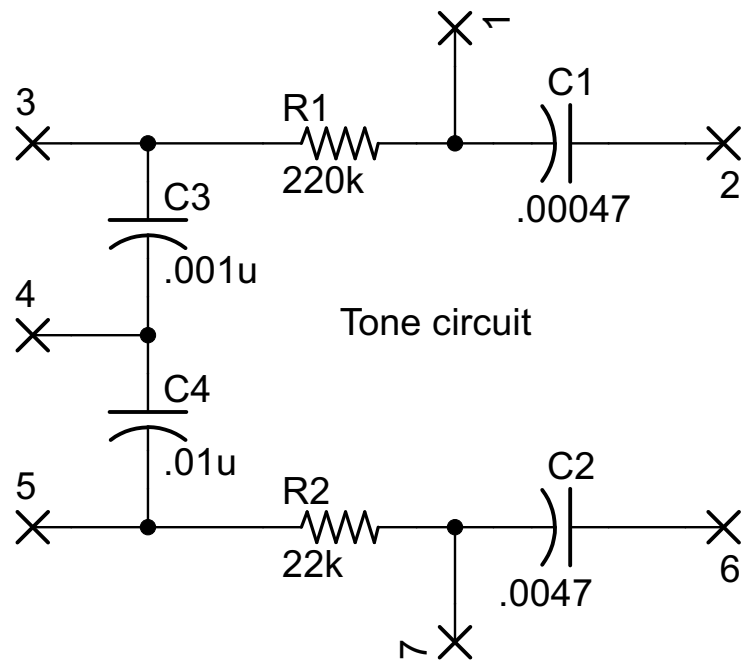
FCN-51-B tone stack 03/12/10 CtG electronics k.b.c.
